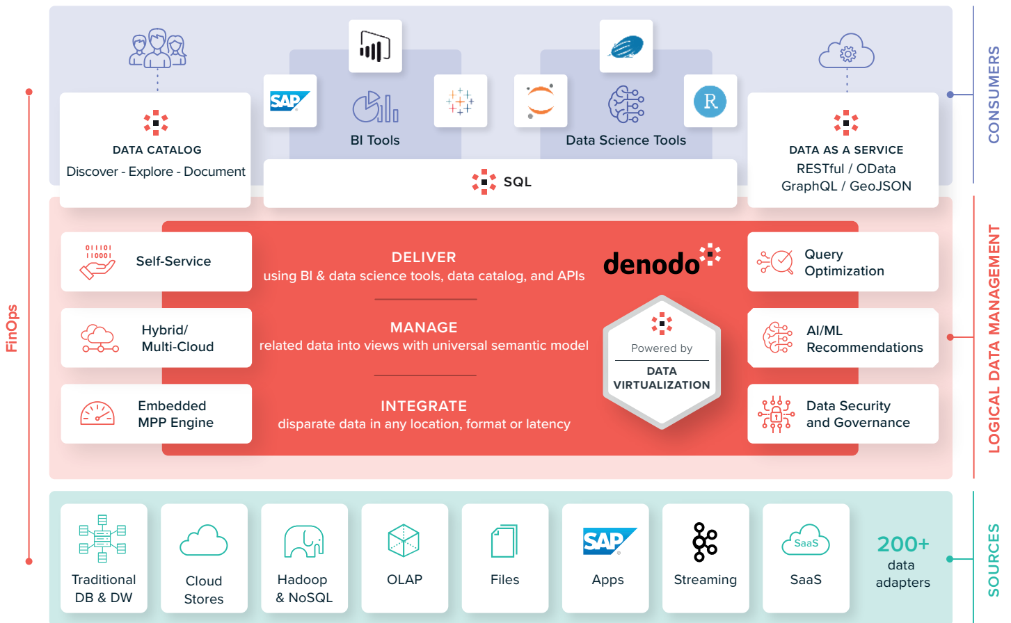
Fig. 1 Denodo Professional Architecture
